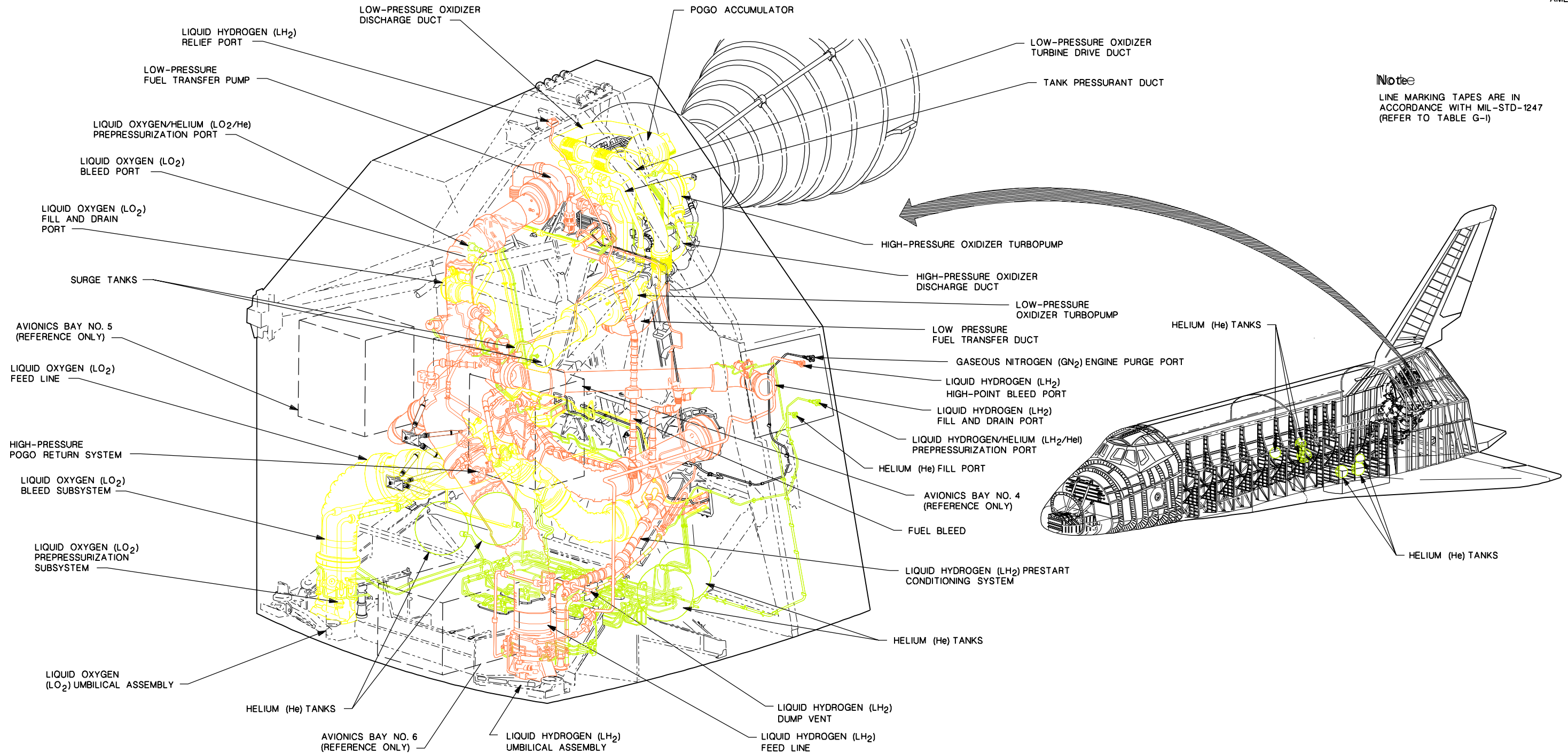
Figure 2-15.- Main propulsion system component/ line locator.
