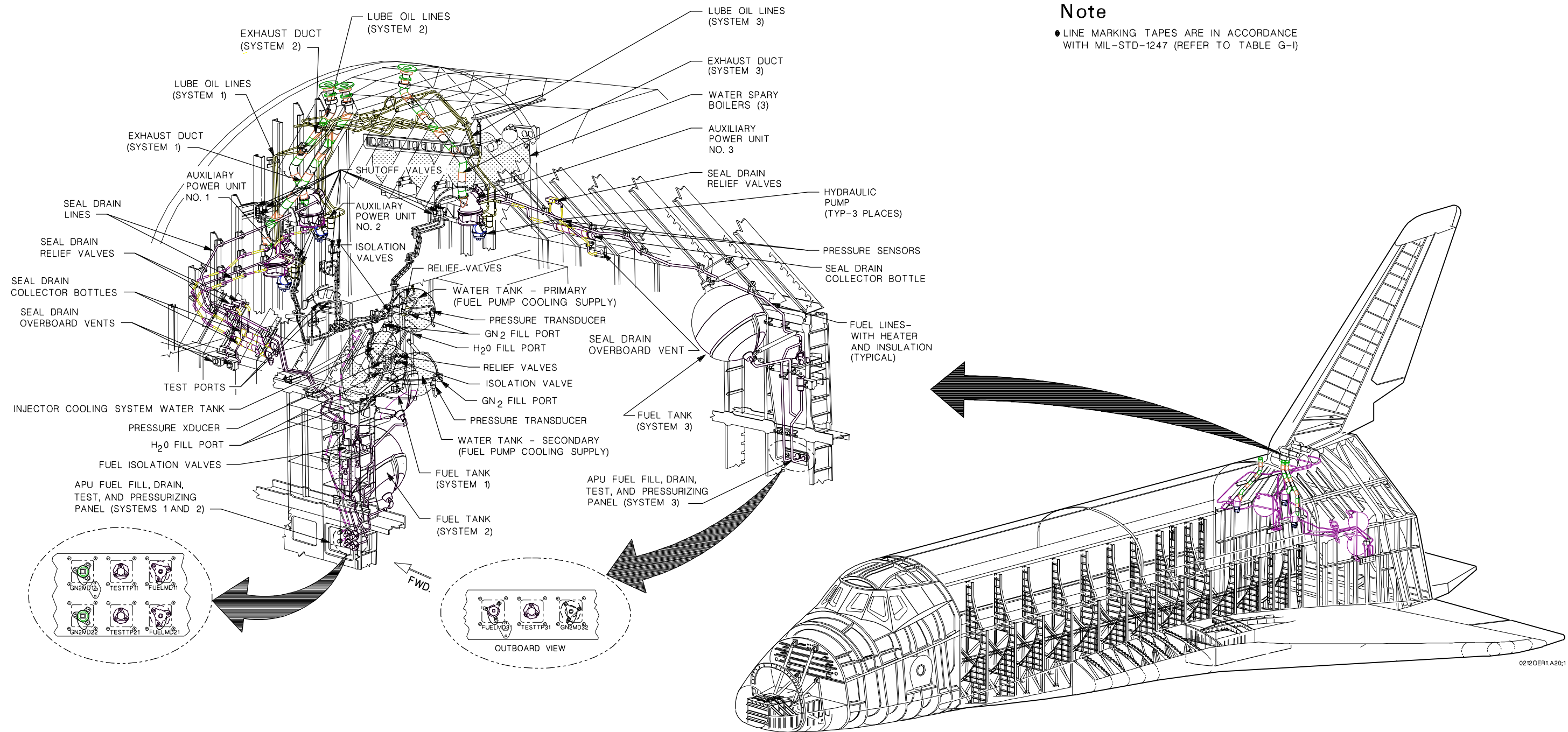
Figure 2-12.- Auxillary power system component/line locator.
