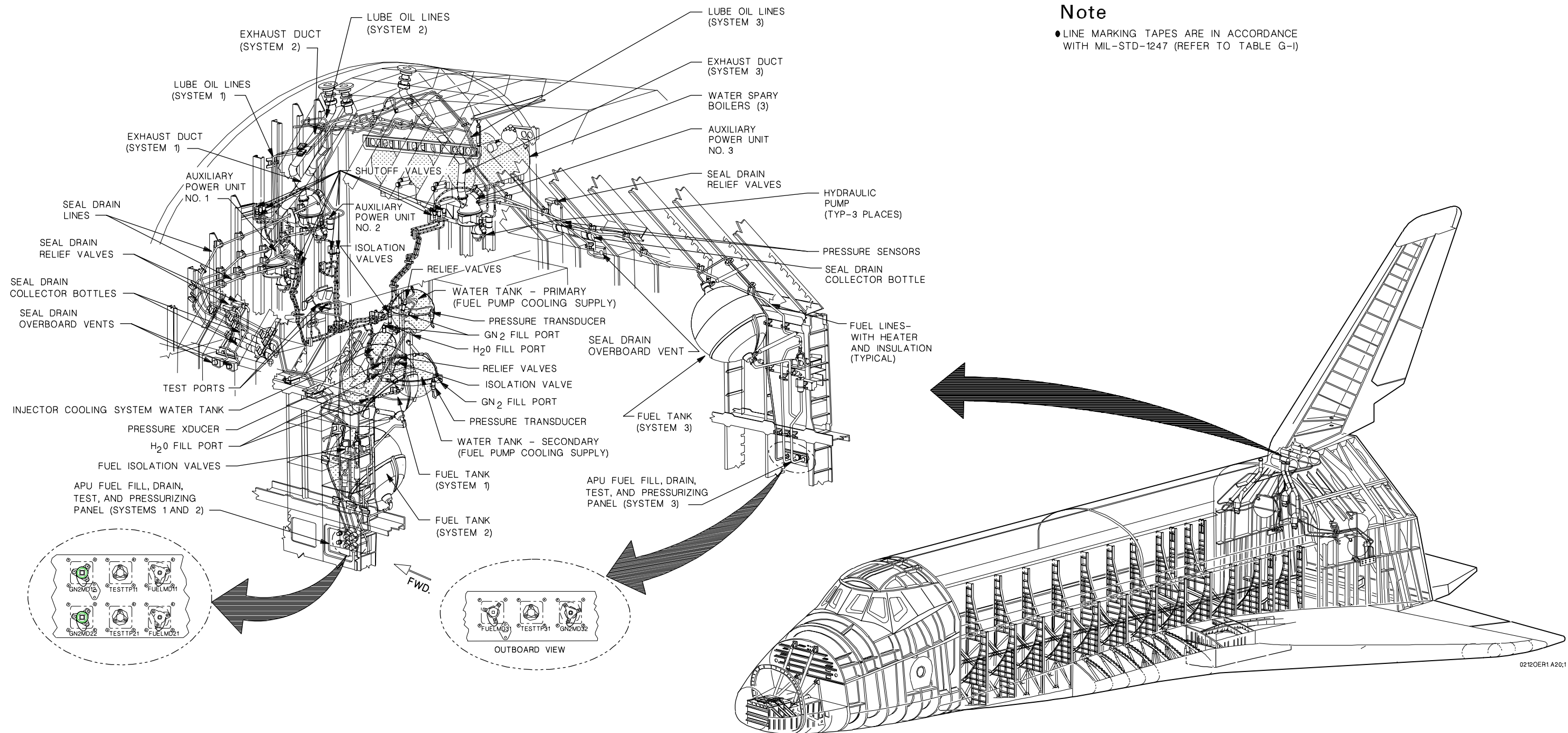
Figure 2-12.- Auxiliary power system component/line locator.
