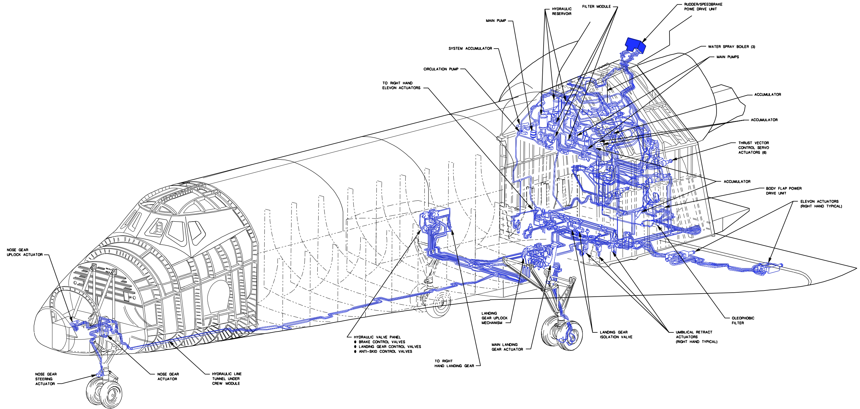
Figure 2-11.- Hydraulic system component/line locator.
