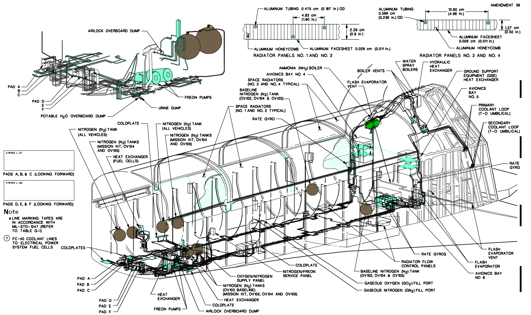
(c) Mid-fuselage and aft-fuselage coolant system Figure 2-10.- Concluded.
