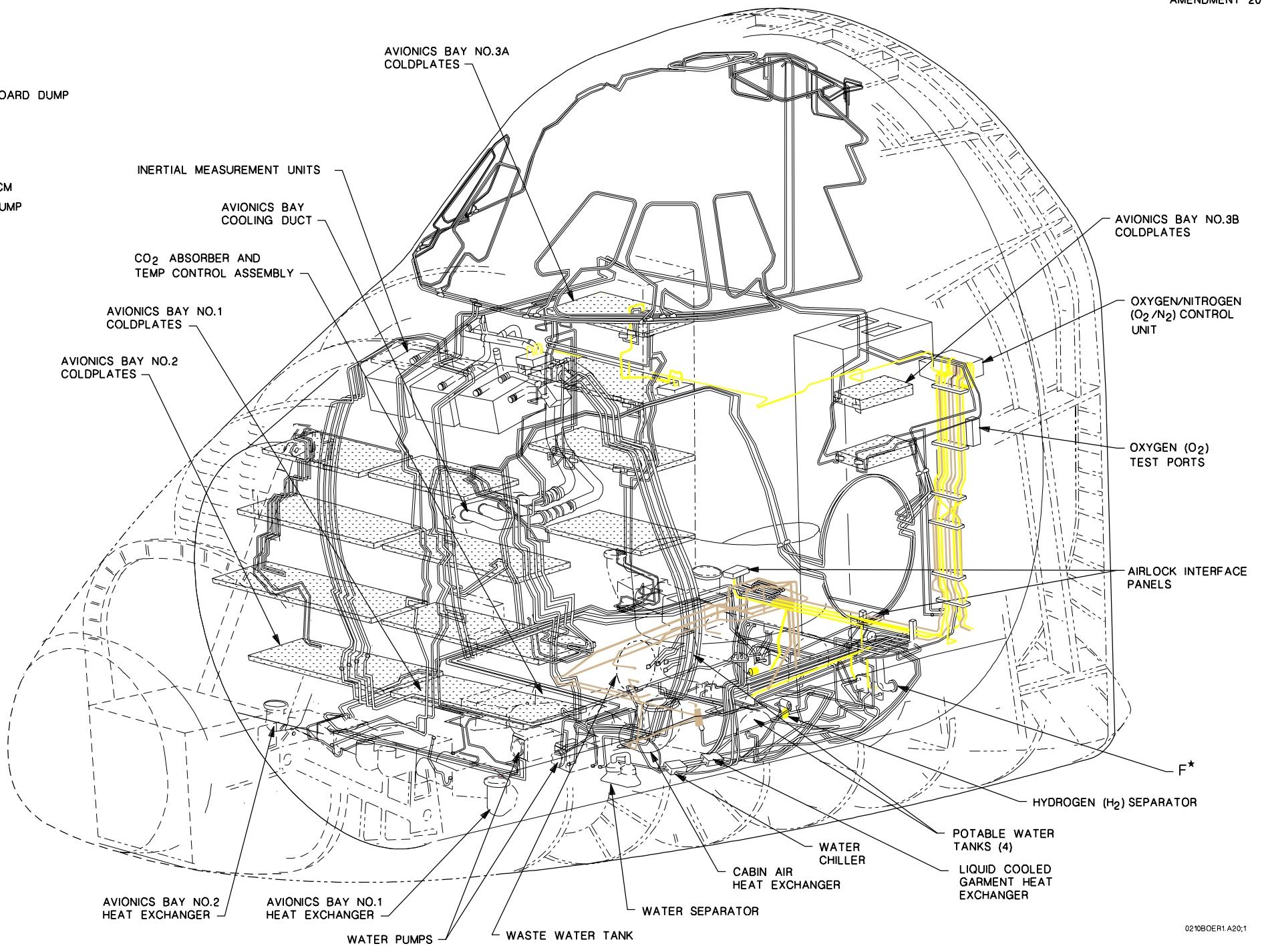
(b) Forward fuselage coolant/air revitalization components.
